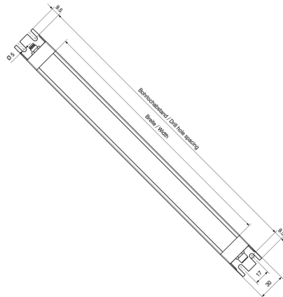
Dimensioned drawing
