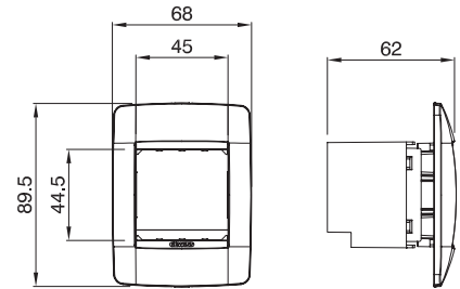
2 POSTI GW 16 712 TB - GW 16 712 TN - GW 16 712 VT
