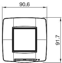
2 POSTI GW 16 702 TB - GW 16 702 TN - GW 16 702 VT
