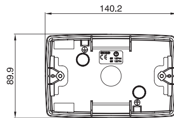
4 POSTI GW 16 744 - GW 16 774
