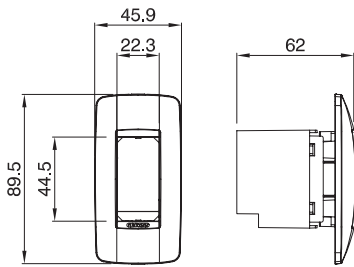
1 POSTO GW 16 711 TB - GW 16 711 TN - GW 16 711 VT
