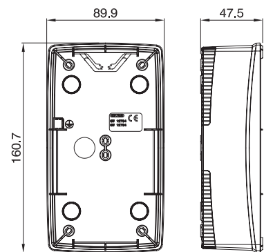
2+2 POSTI VERT. GW 16 754 - GW 16 784
