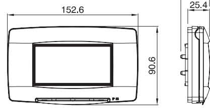
4 POSTI GW 16 704 TB - GW 16 704 TN - GW 16 704 VT
