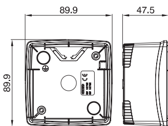
2 POSTI GW 16 752 - GW 16 782
