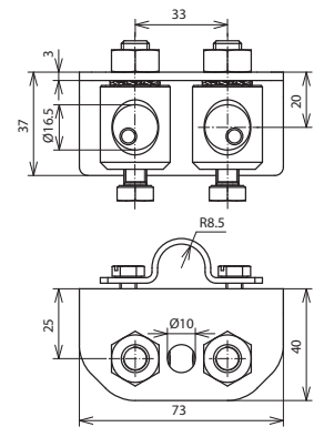
Maßbild AD WAS 16 BB16 V2A
