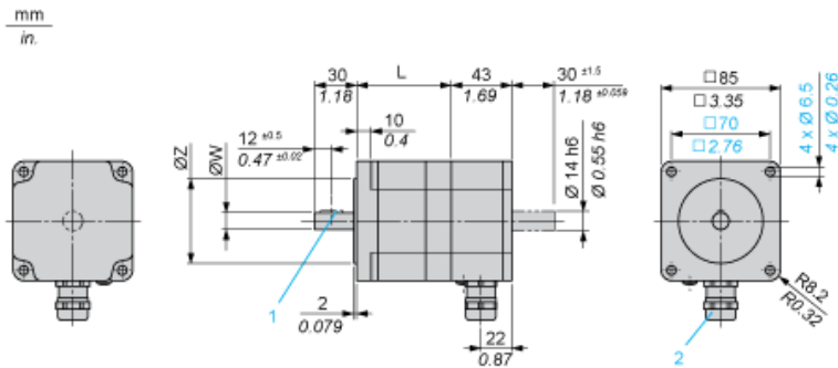
Abmessungen in mm
