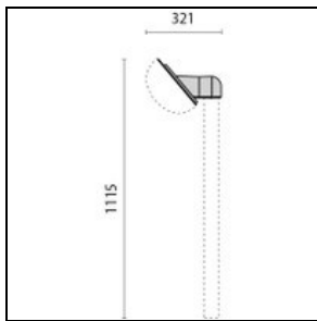
000800 Angled bracket for 42 mm post ■ BK-81 / Black
