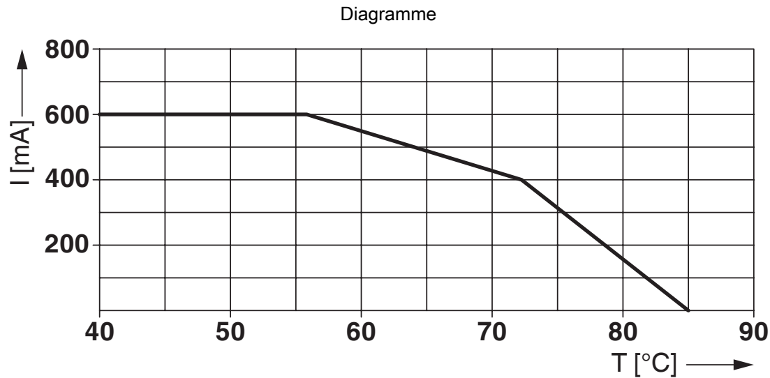
Diagramme Derating for Ex-areas (Zone 2, EX ec)
