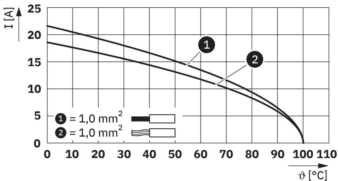
Diagrama derating para 1,0 mm 2
