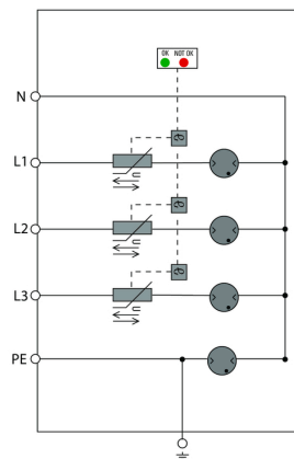
Circuit diagram
