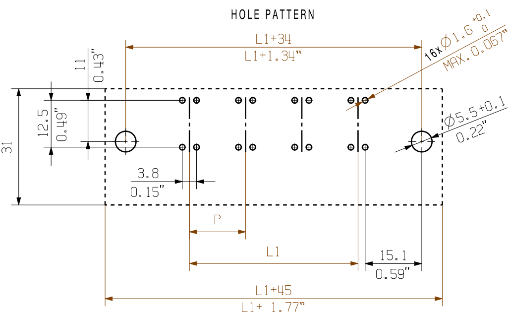
HOLE PATTERN
