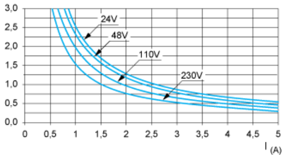
Curve AC12
