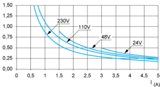
Curve AC15
