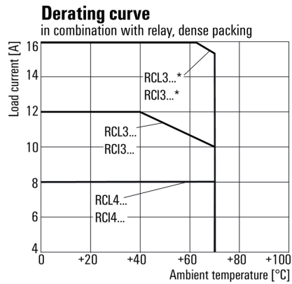
Deratingkurve
