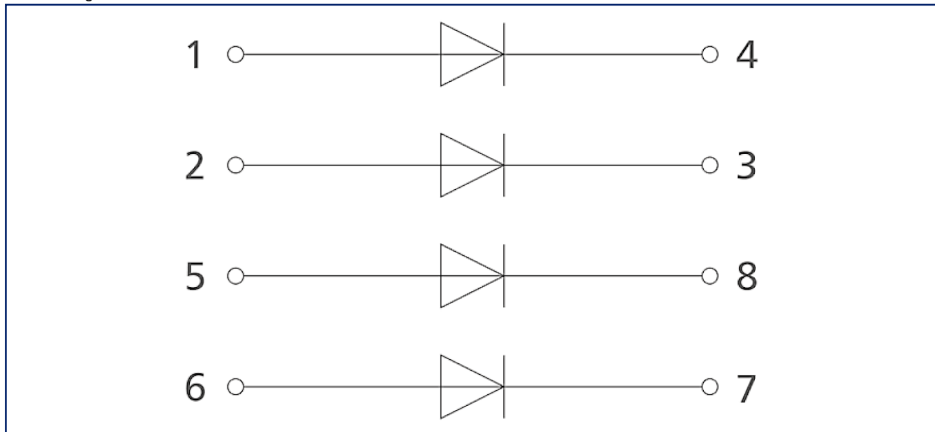
Circuit diagram
