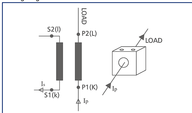
Wiring diagram
