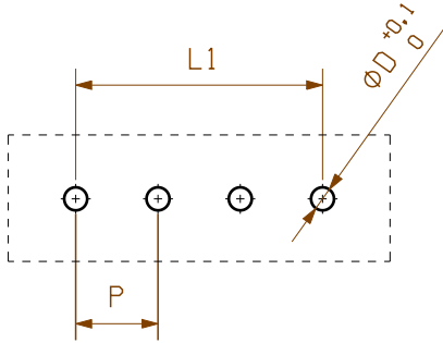
HOLE PATTERN
