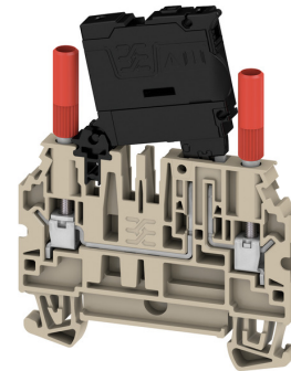
Version with hollow screw for testing
