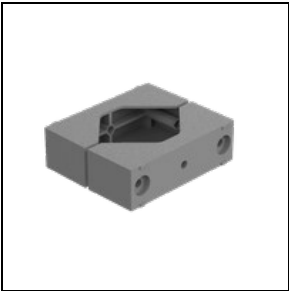
14047194 Gliding support made of painted aluminium for the installation on 60-76 mm Ø posts. 2 opposed luminaires ■ GR-g4 / Metallic grey
