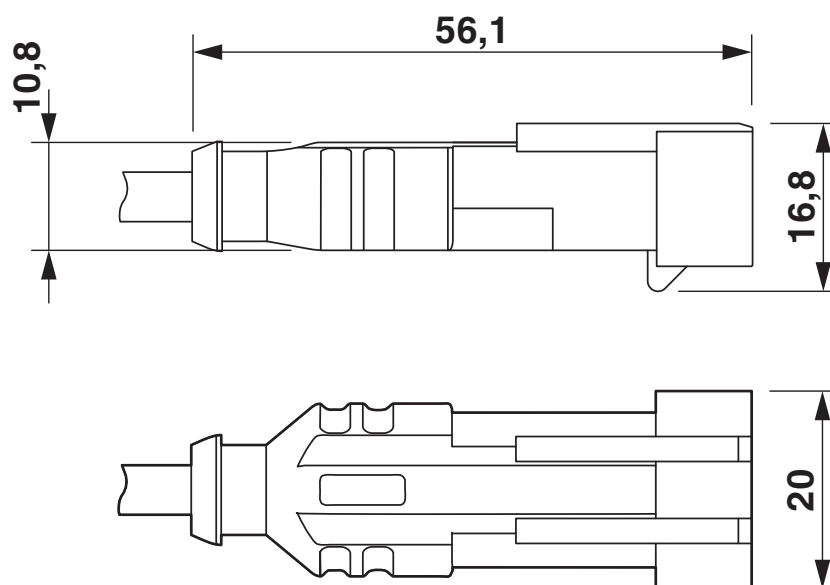
Superseal, conector, vista superior y lateral
