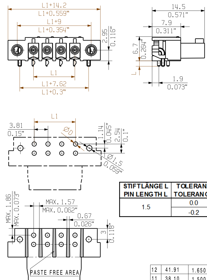
BCL-SMT 3.81/.../90LFI 1.5...
