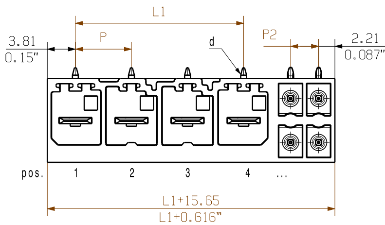
SV-SMT 7.62HP/04/270G...SC04
