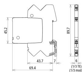
Schema dimensioni BCO ML2 BD HC5A 24
