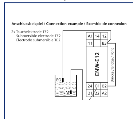
Connection example
