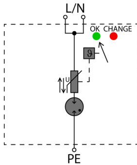
Schematic circuit diagram
