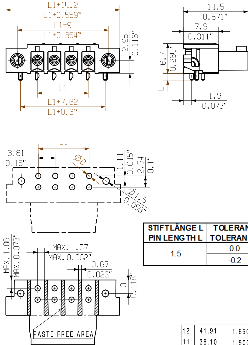
BCL-SMT 3.81/.../90LF 1.5...
