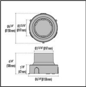
3109879 Controcassa CRICKET+ 10
