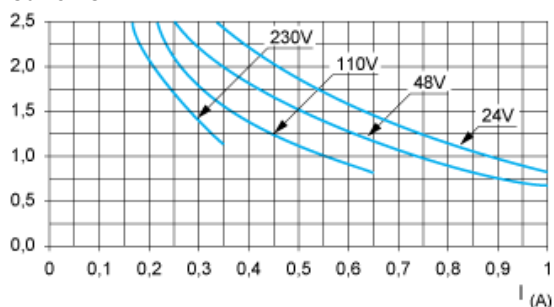
Curve AC14
