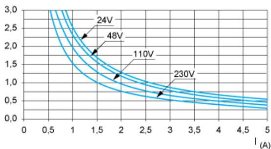
Curve AC12
