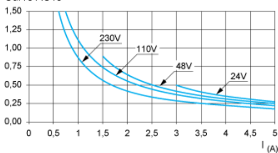
Curve AC15
