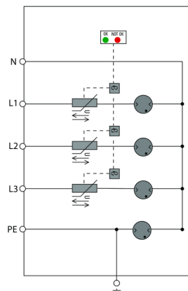
Circuit diagram
