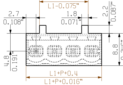
MIN. FRONT PLATE CUT-OUT
