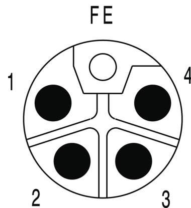
Plug
