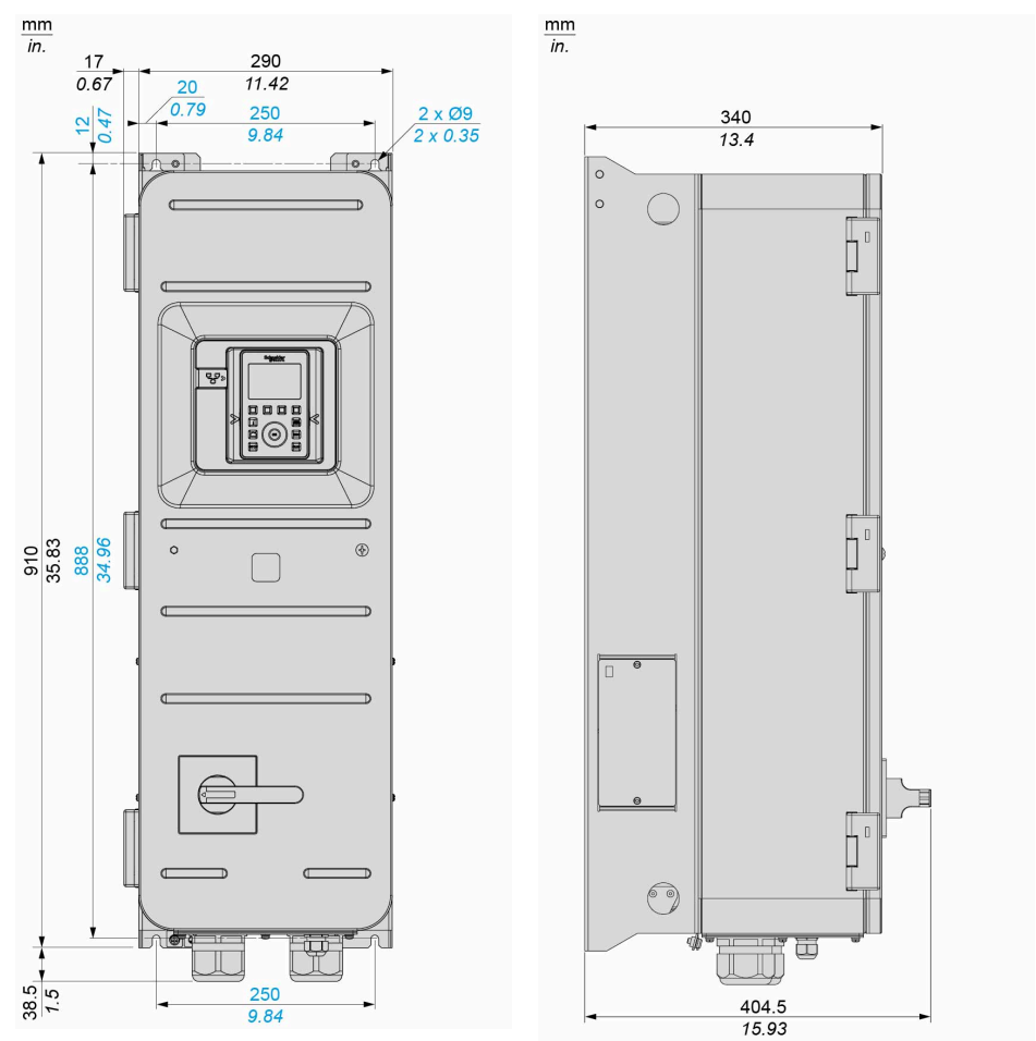
IP55 / UL Type 1 Drive With Disconnect Switch - Front and Side view
