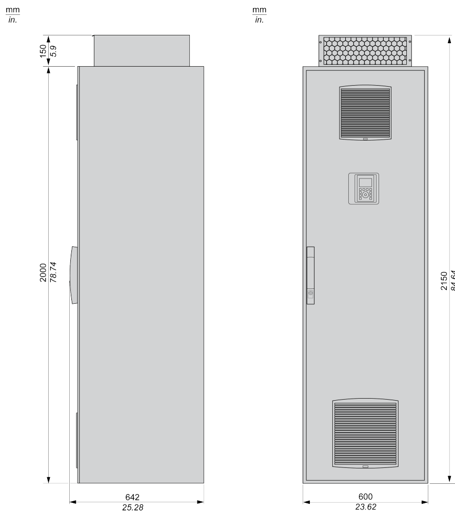
IP 21 Drives - Side and Front View
