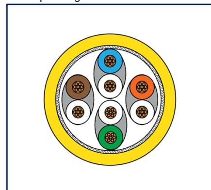
Principle diagram
