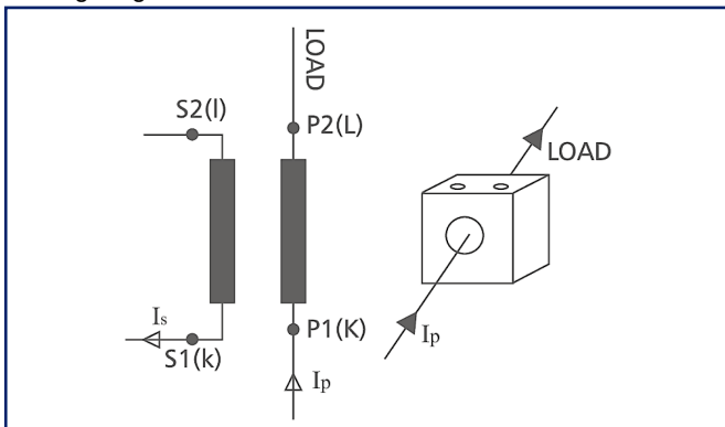
Wiring diagram
