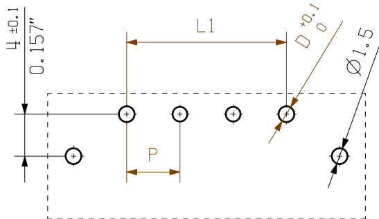
hole pattern
