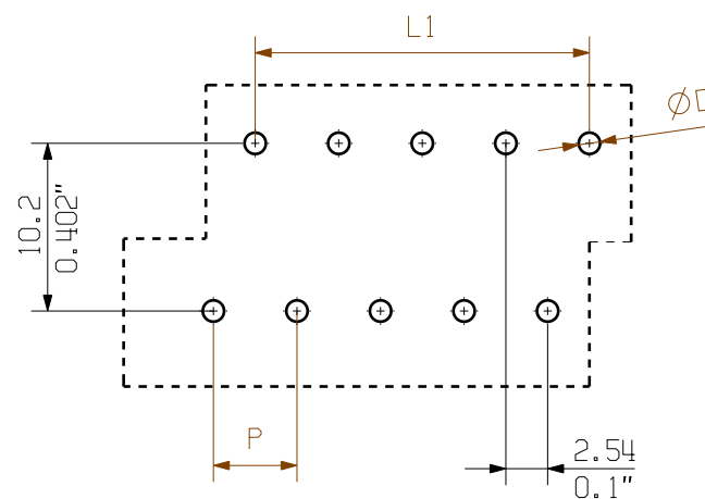
PCB LAYOUT
