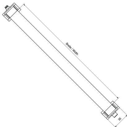
Dimensioned drawing
