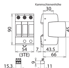
Dimensioni DG M YPV 1200 FM - old
