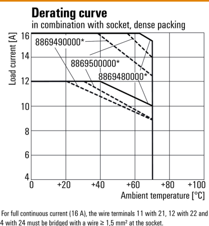
Relay in combination with base
