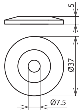
Maßbild AS 37 5 B7.5 UVS K BR
